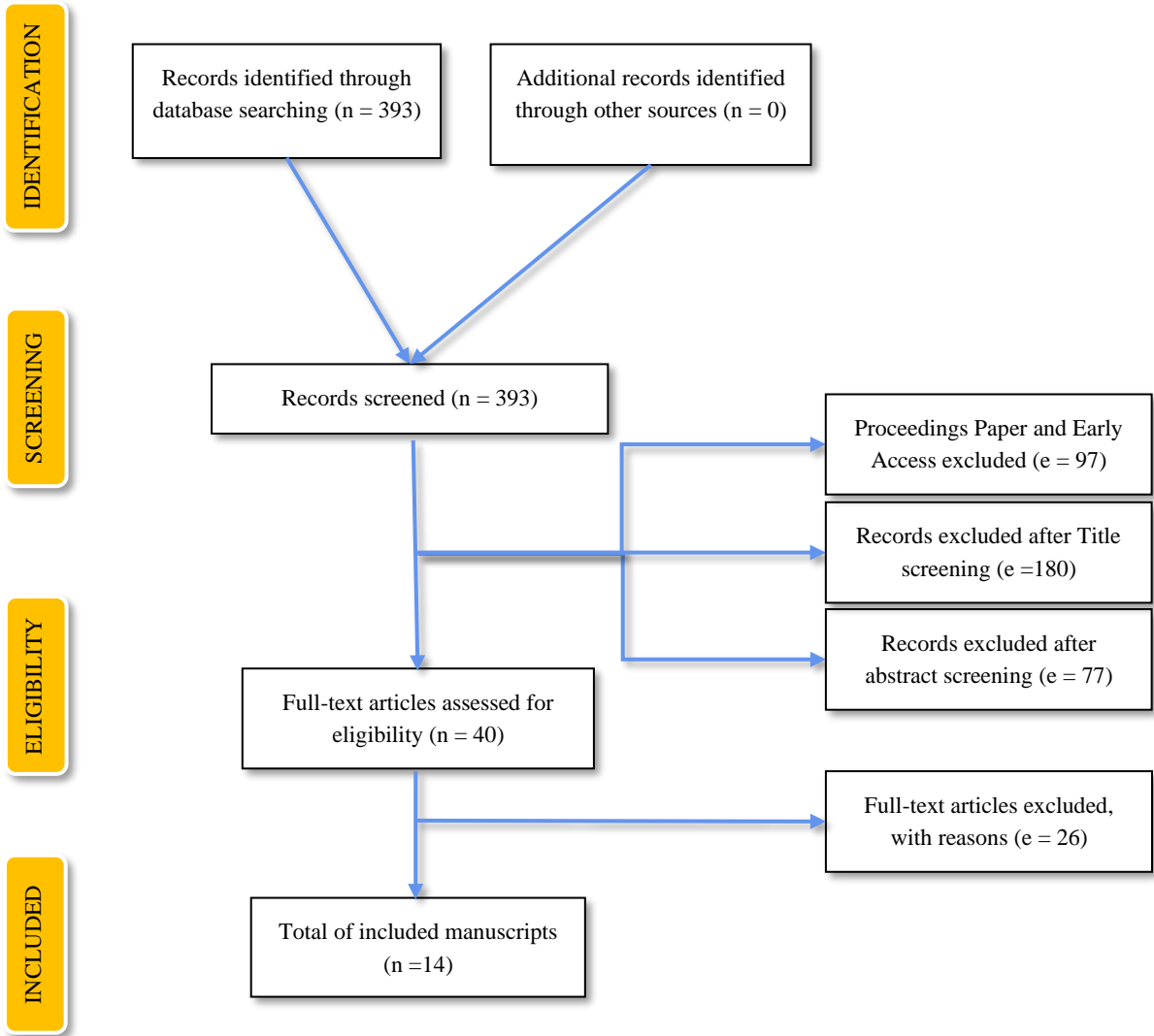
Figure 13 PRISMA Diagram
